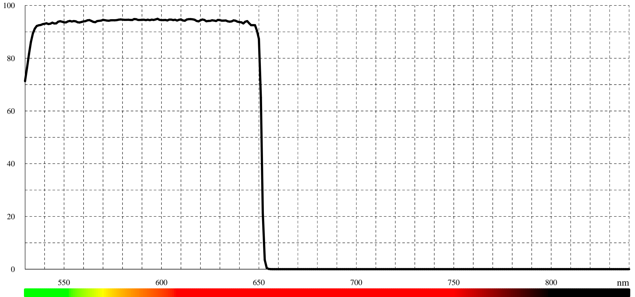
Typical transmission for SP 647 (LF101853)
