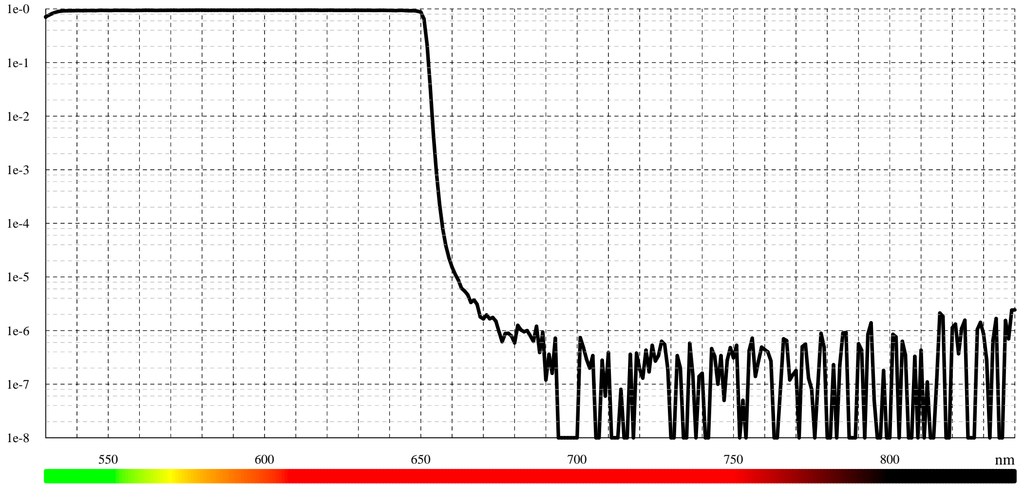
Typical blocking for SP 647 (LF101853)
