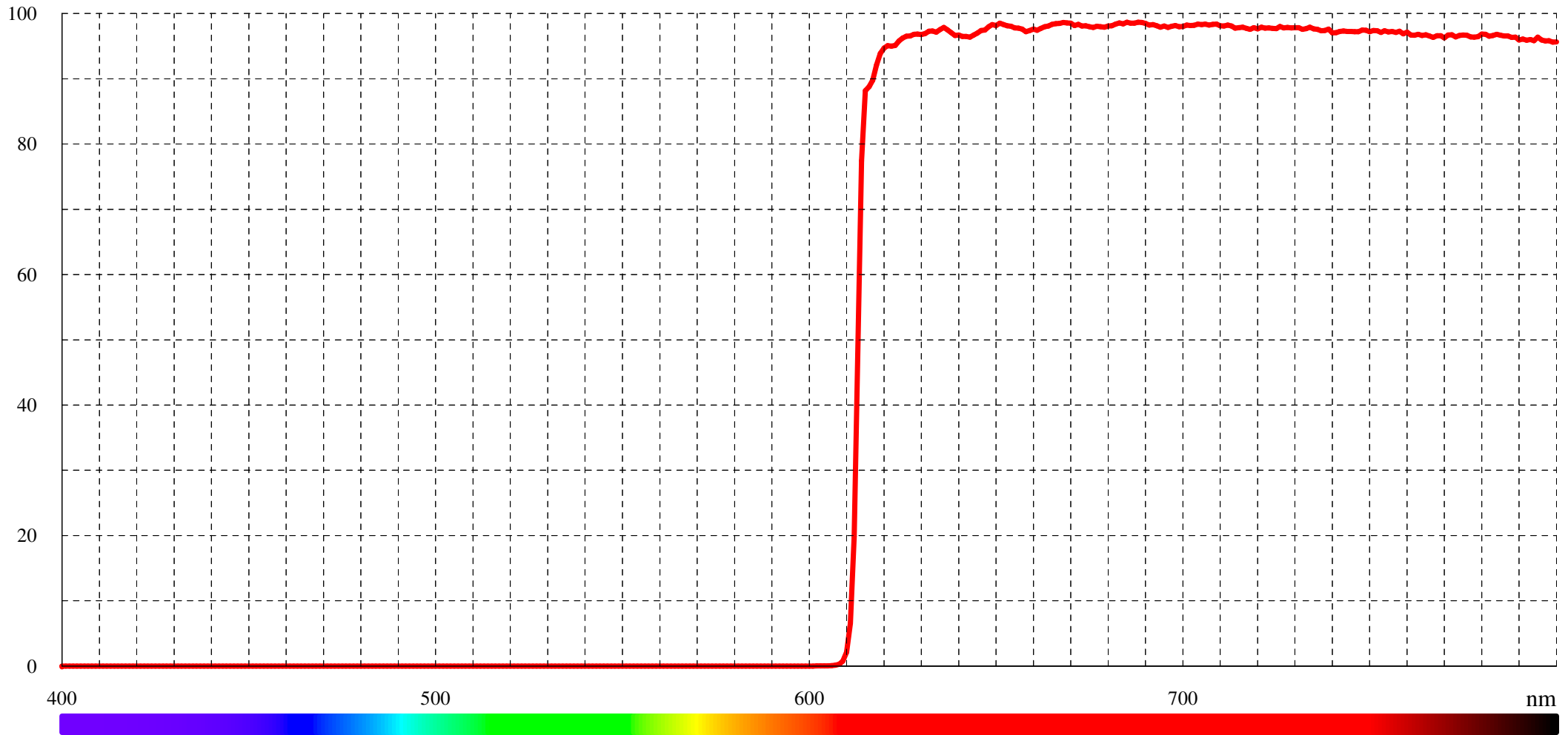
Typical transmission for LP 615 (LF101596)
