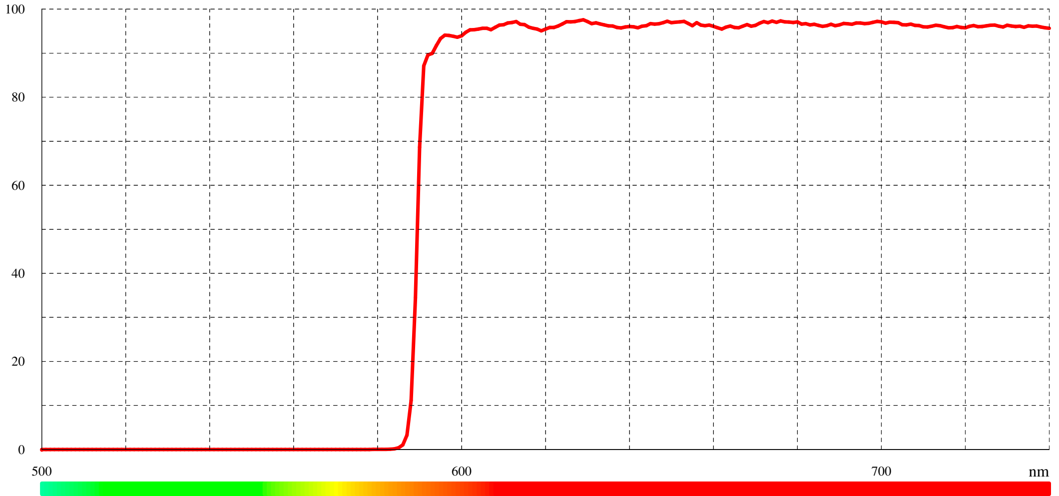
Typical transmission for LP 590 (LF101579)
