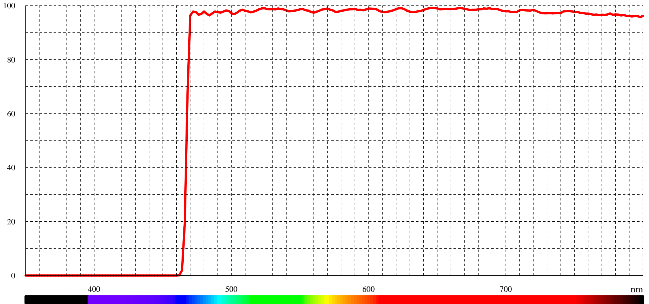
Typical transmission for LP 470 (LF101834)
