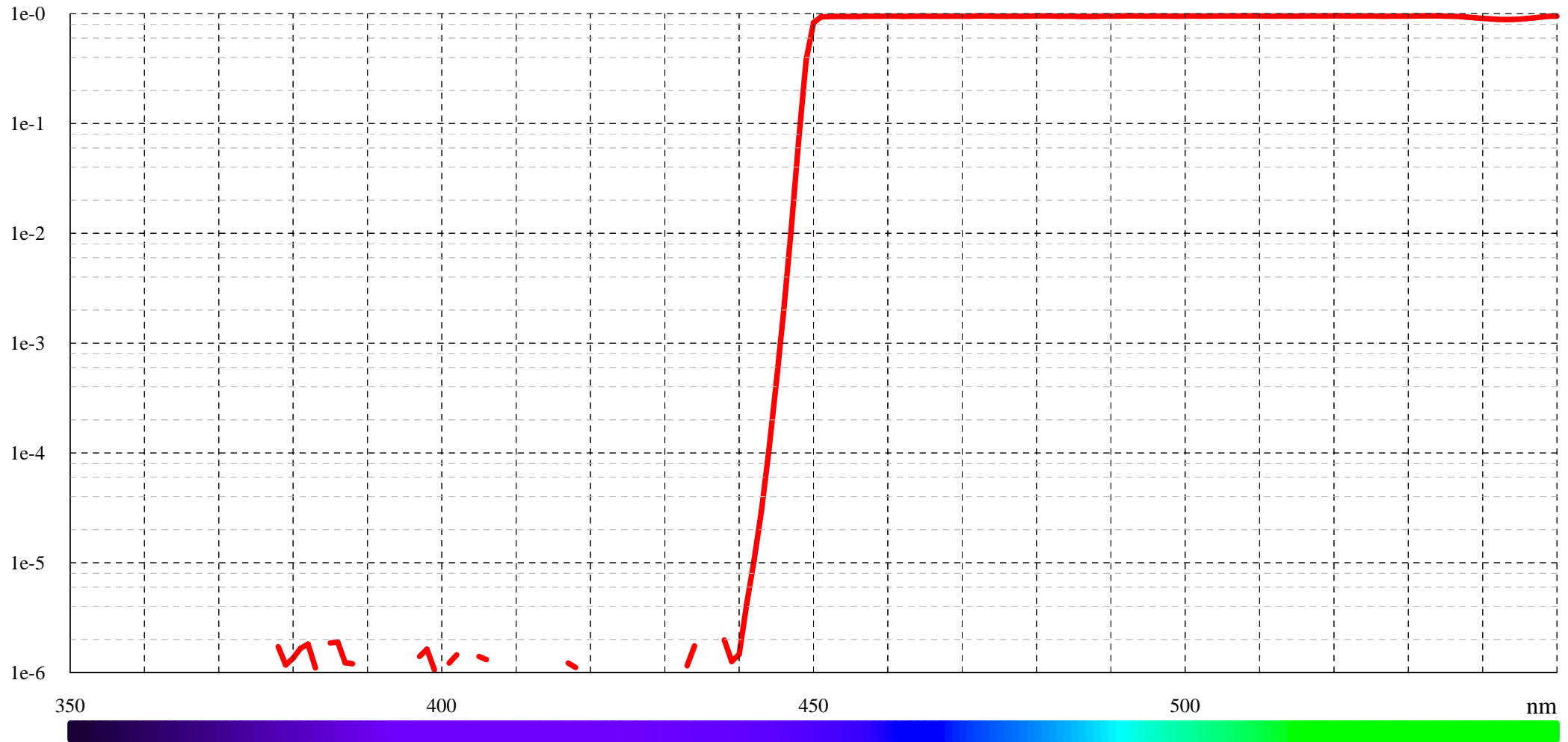
Typical transmission of LP450 (LF101859)
