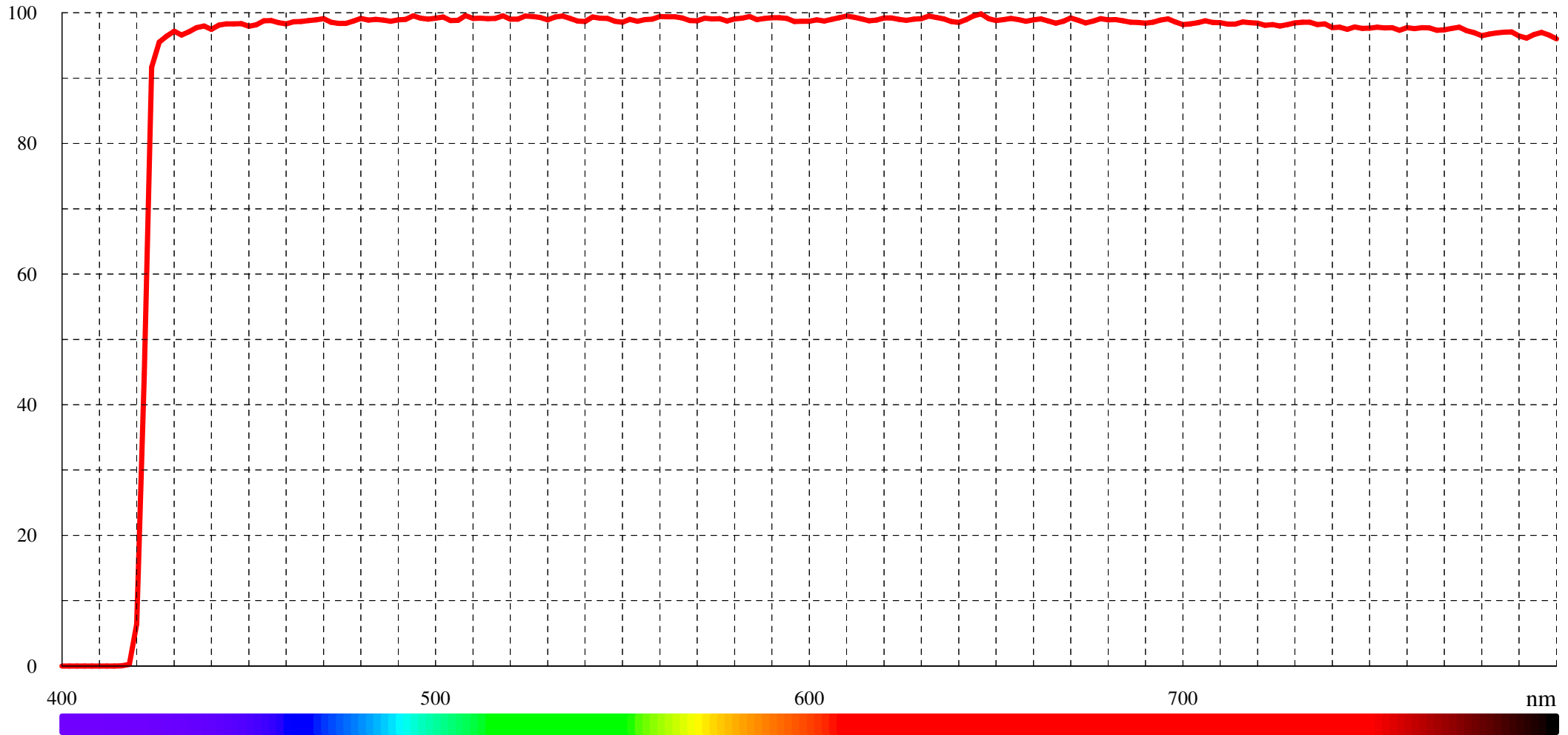
Typical transmission for LP 420 (LF101642)
