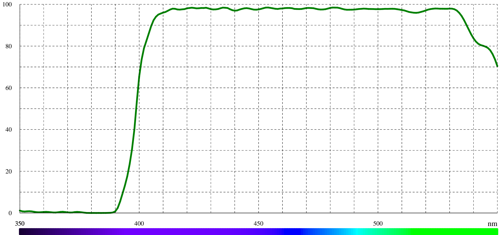
Typical transmission for DCLP 403 (LF101833)
