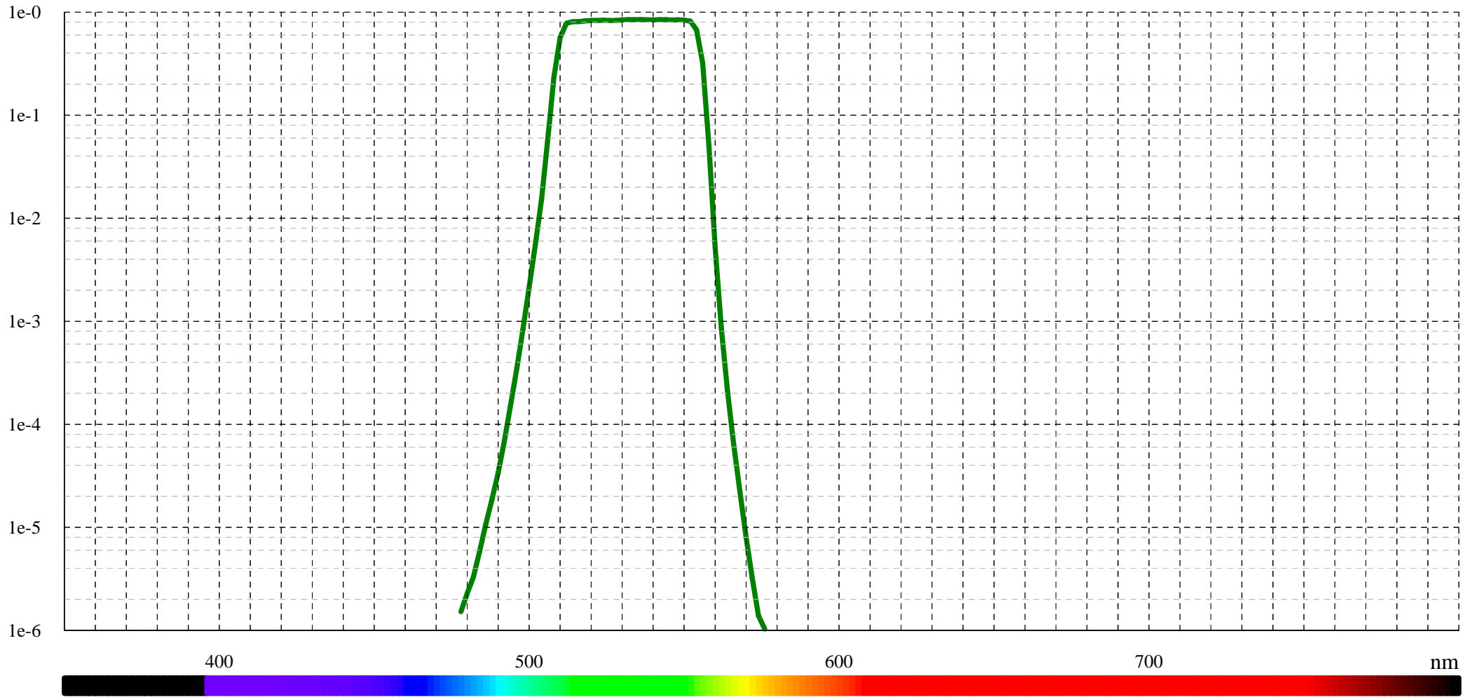
Typical blocking for BP 535/50 (LF101752)
