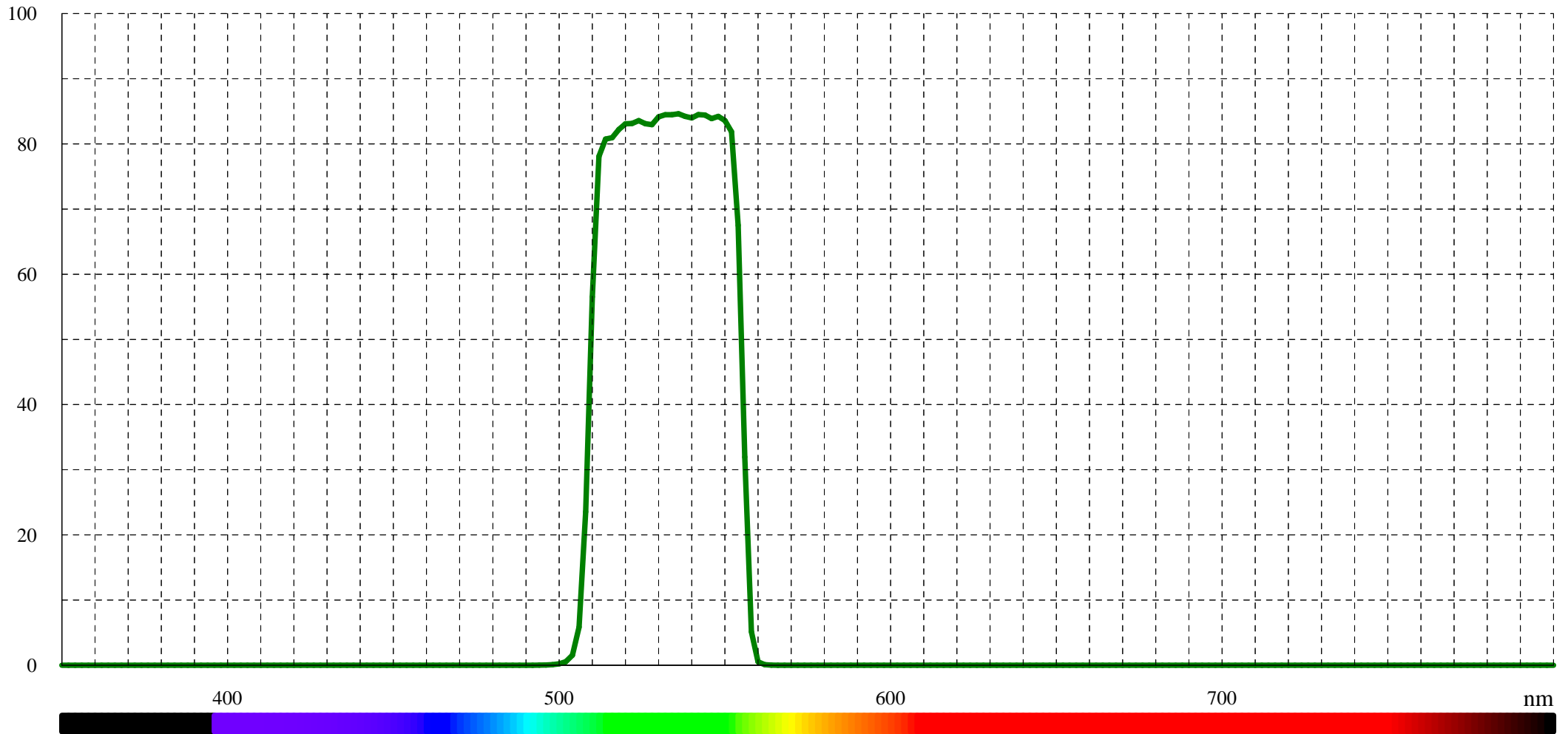
Typical transmission for BP 535/50 (LF101752)
