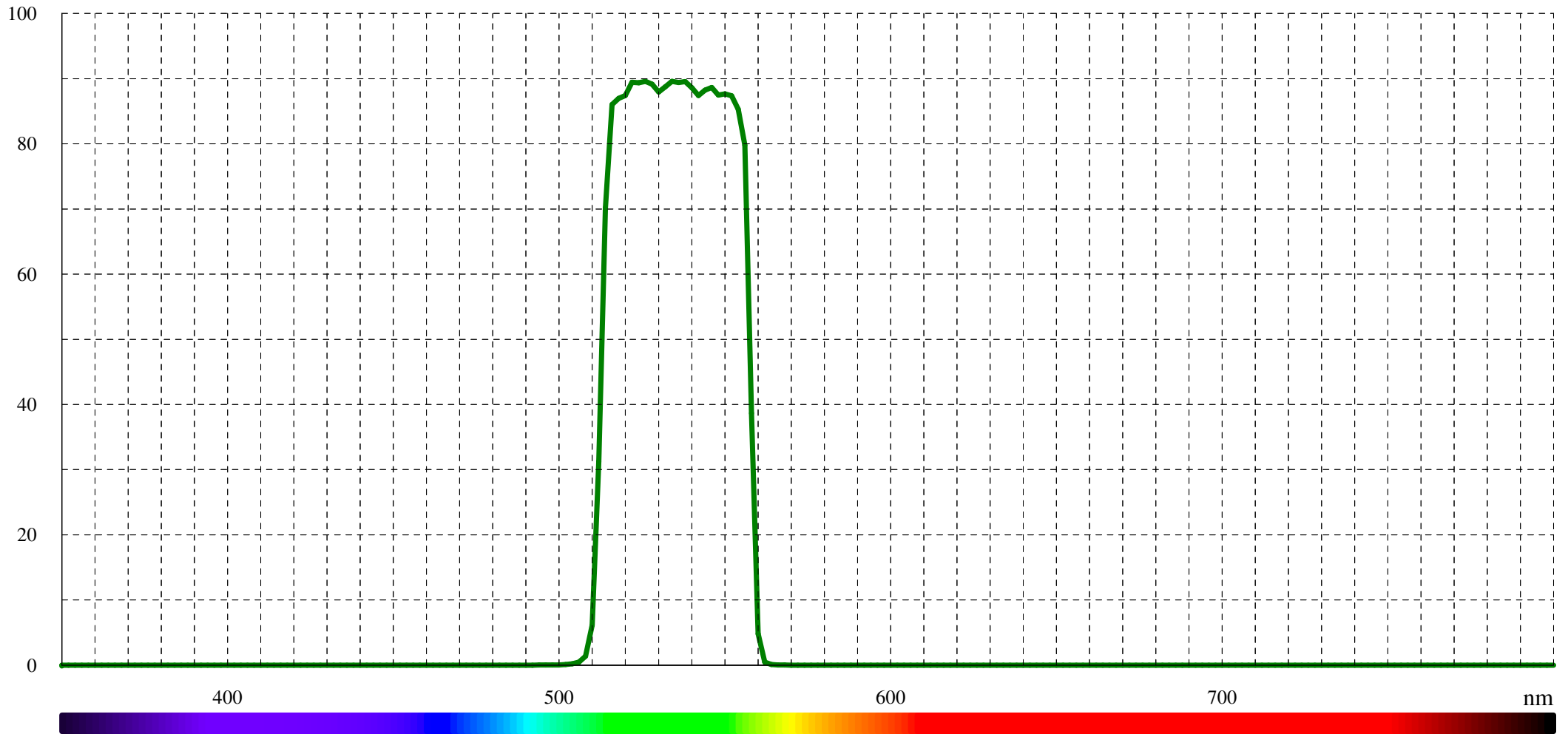
Typical transmission for BP 535/45 (LF101668)
