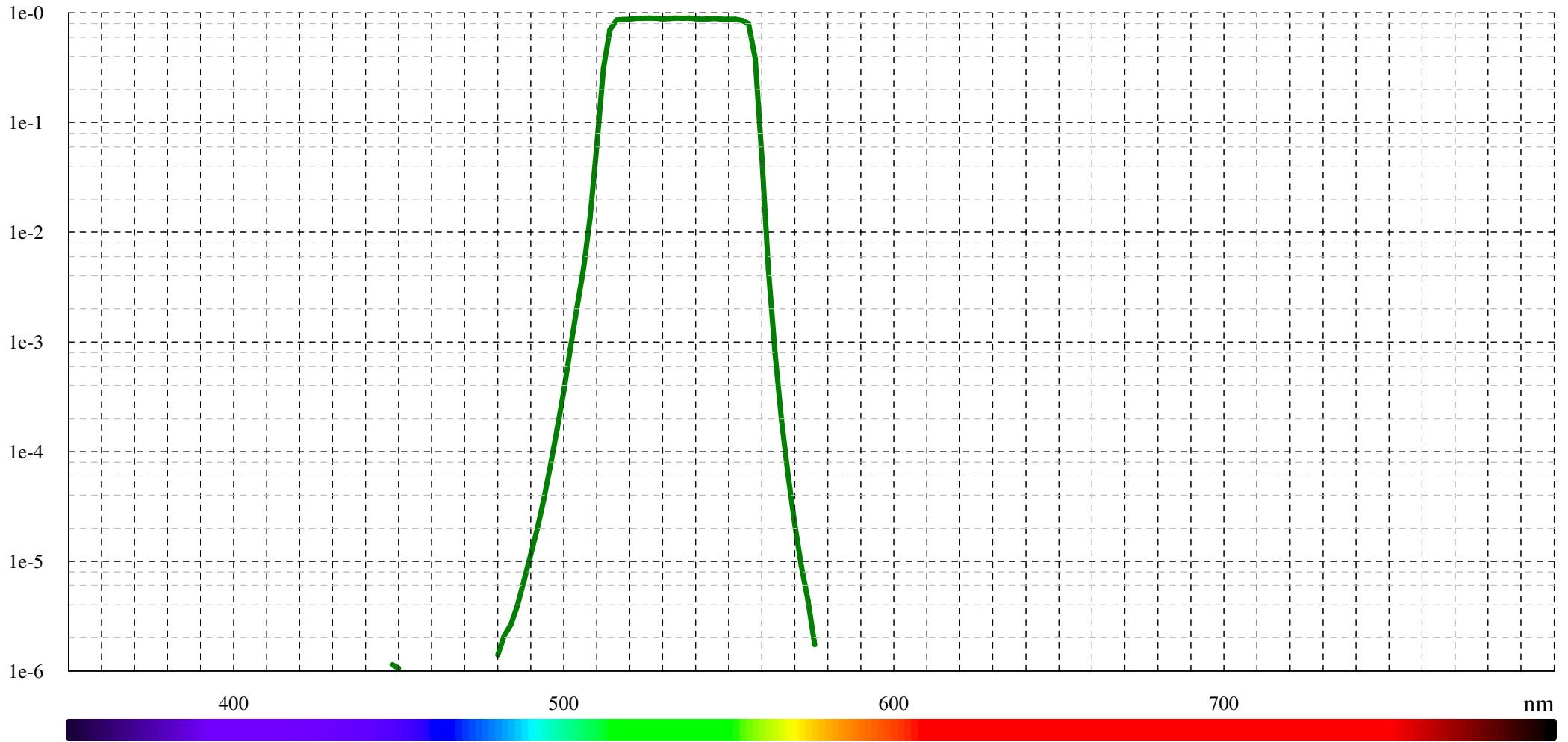
Typical blocking for BP 535/45 (LF101668)
