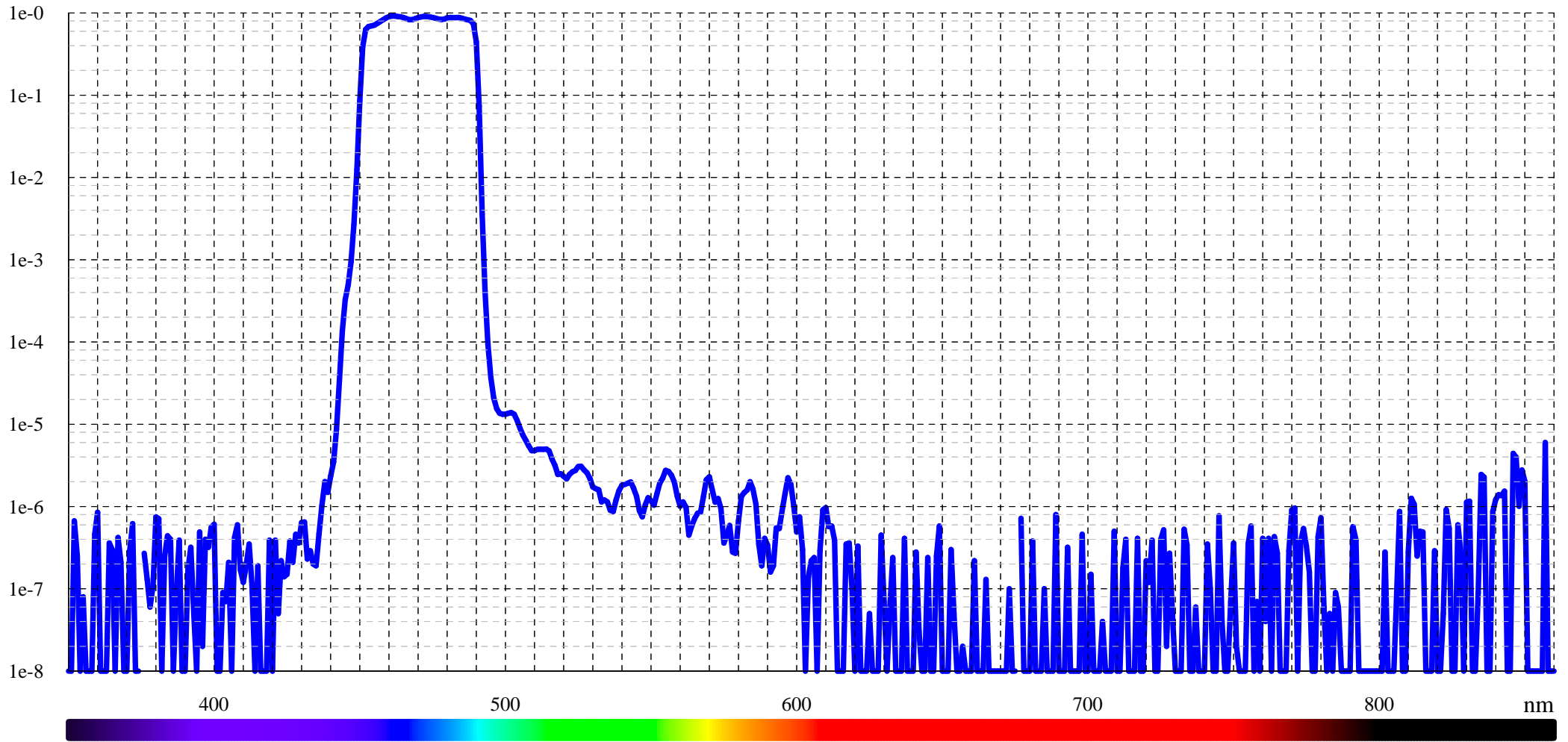
Typical transmission for BP 470/40 (LF102017)
